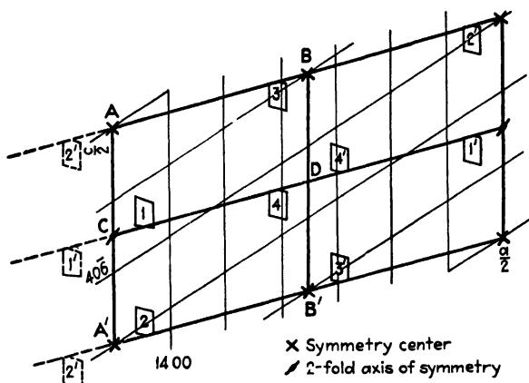
FIG. 4.—Projection on the (010) plane of regions permitted to Si. (Only one-fourth the base of the unit-crystal is shown).
